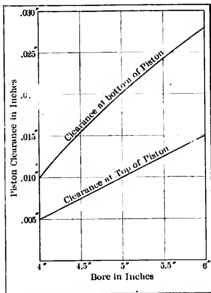
Fig. 1—Curves of piston clearance, showing the correct amount at top and bottom
